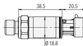
8252.XX.XXXX.51.XX.XX
