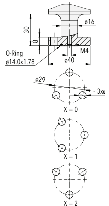
87x6.XX.220x.XX.XX.XX.XX Axial flanged connection
