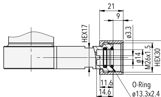
87x6.XX.2XE2.XX.XX.XX.XX Raccord radial DN8
