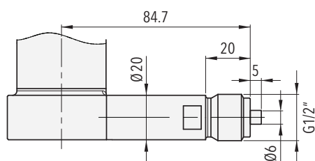
87x6.XX.1030.XX.XX.XX.XX Raccord fileté radial G1/2"
