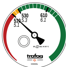
Partial indicator dial with sectors according to customer specification
