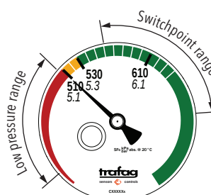
Full range indicator dial according to customer specifications
